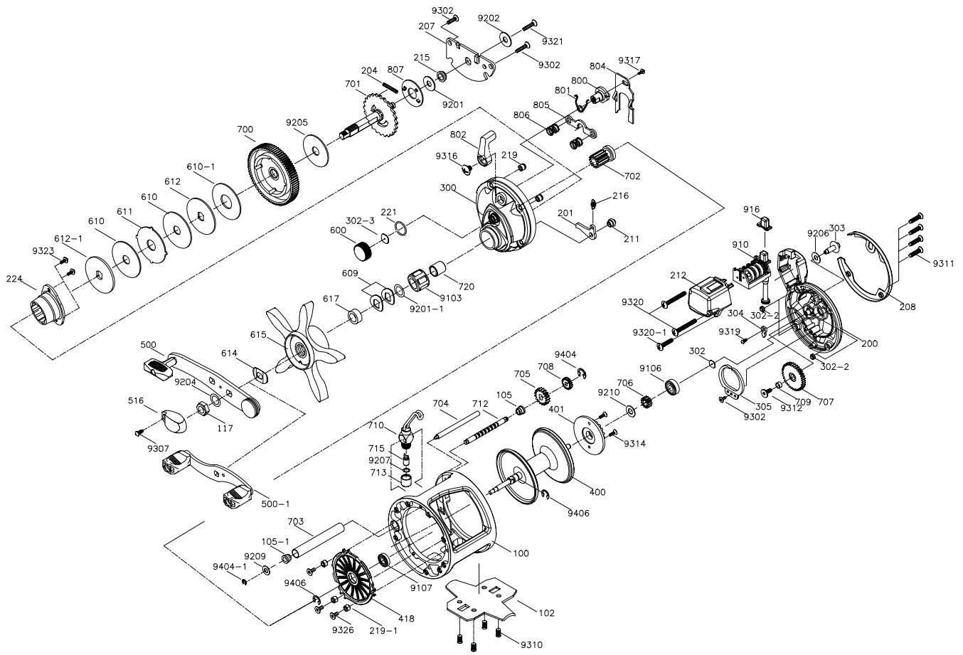
DMG - 20L (2 of 2) Spare Parts
